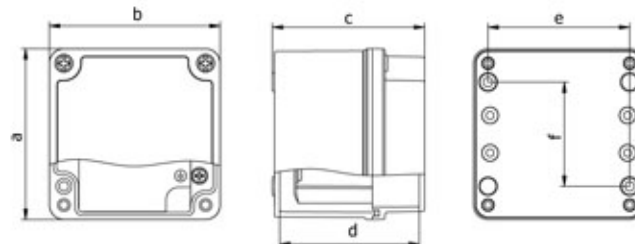
402554 ALÜMİNYUM BUAT (80 x 80 x 73 mm) Aluminium Enclosure
