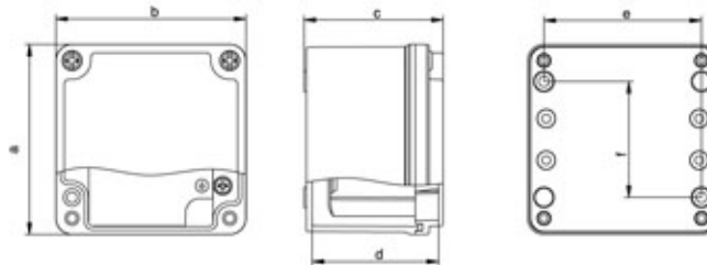
402503 ALÜMİNYUM BUAT (65 x 100 x 40 mm) Aluminium Enclosure
