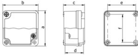
402502 ALÜMİNYUM BUAT (65 x 65 x 40 mm) Aluminium Enclosure
