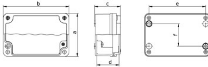
402502 ALÜMİNYUM BUAT (65 x 65 x 40 mm) Aluminium Enclosure
